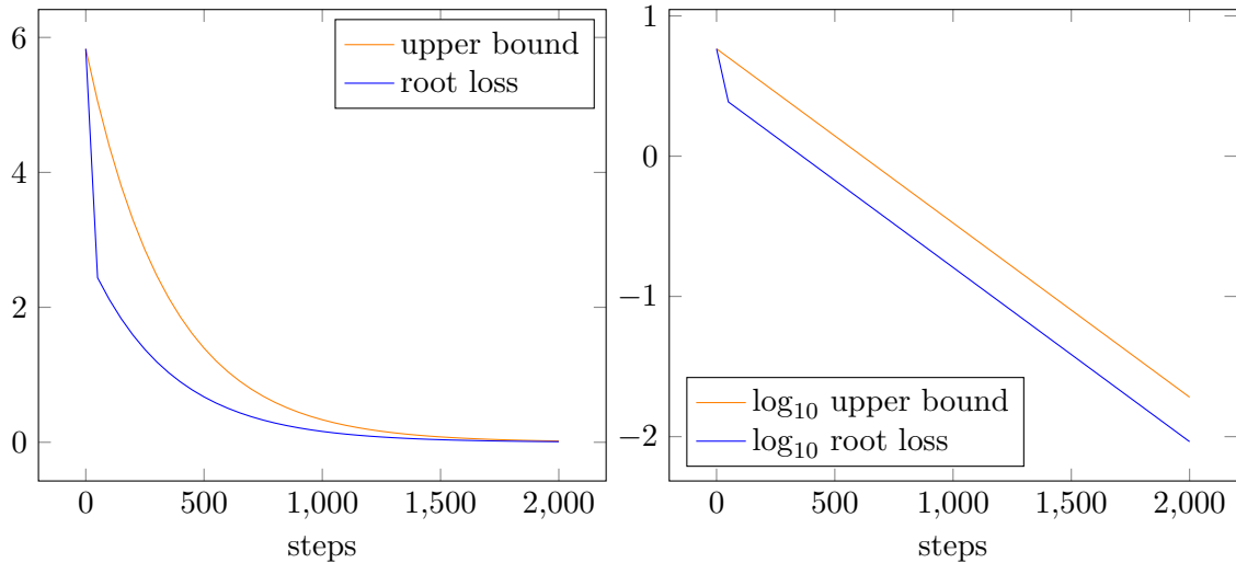
FIGURE 1: Loss as a function of time at (a) regular (b) regular-log scale.
