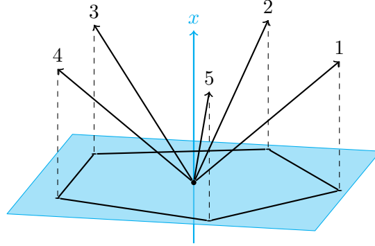
FIGURE 4: Embedding of the 5-cycle and its projection to the subspace spanned by eigenvectors \mathbf{v}_2 and \mathbf{v}_3 .
