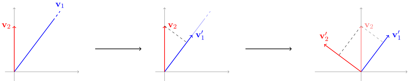
FIGURE 5: Gram-Schmidt orthogonalization of \mathbf{v}_1, \mathbf{v}_2 .
