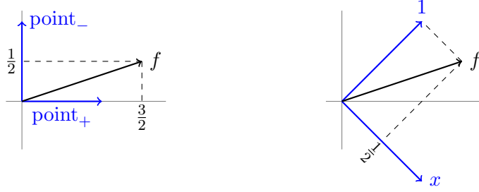
FIGURE 1: The Fourier representation as a change of basis.
